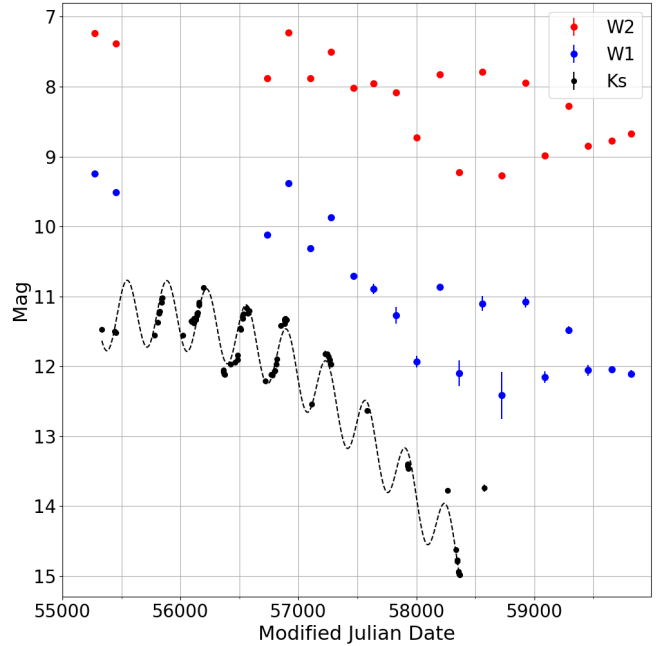
Figure F2. VVV and WISE light curves of source 163. These appears to be a combination of pulsation and a slower, extinction-driven dip. The dashed line shows a simple model fit, see main text. The background grid aids comparison of the amplitude of pulsation in the three filters.
