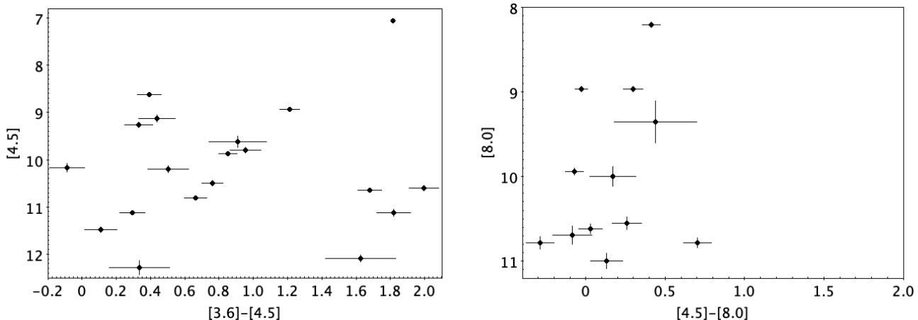
Figure 11. Spitzer /IRAC colour-magnitude diagrams for the dipping giants. ( left panel ): [3.6]–[4.5] vs. [4.5] plot for 19 sources. ( right panel ): [4.5]–[8.0] vs. [8.0] plot for 12 sources, with the abscissa scaled to emphasise the relatively blue nature of the population in this colour, which is almost independent of extinction. Many sources have [3.6]–[4.5] < 1, also indicating little emission by hot dust at the time of the GLIMPSE-II survey in 2005 to 2006, but hot dust is required to explain some sources with [3.6]–[4.5] > 1.
