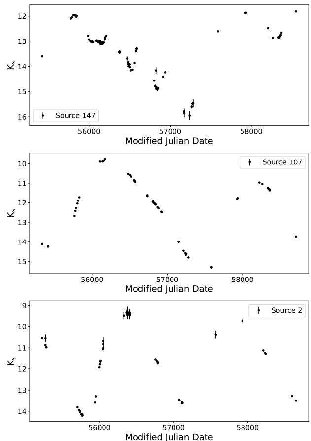
Figure F1. VVV light curves of three notable LPVs. Source 147 shows a \sim 3.5 mag fading trend over 4 years before recovering. Source 107 and source 2 have the highest amplitudes of pulsation in the LPV sample, \sim 5 mag in K_s .
