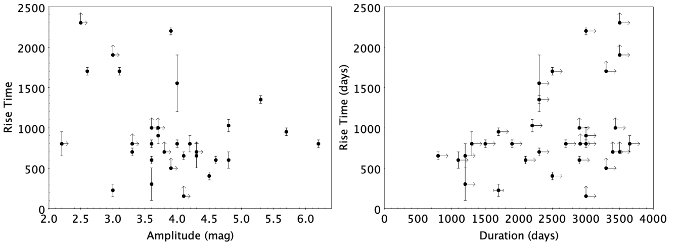
Figure 3. Rise time plotted against amplitude (left panel) and outburst duration (right panel) for 32 classic events drawn from this work and earlier VVV discoveries. Typical rise times are 600 to 1000 days, though there are faster rises and slower rises. Durations are typically lower limits since the events continued beyond 2019.
