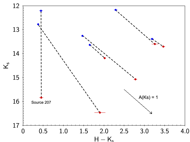
Figure E2. K_s vs. H - K_s colour-magnitude diagram for six of the dipping YSOs. Blue and red points correspond to the brightest and faintest available epochs of multi-filter data, respectively. Elements of a pair are connected by dashed lines. The changes are roughly parallel to the extinction vector in most cases. One source is clearly different: source 207 (the candidate KH15D-like object in the Lagoon Nebular Cluster) shows negligible colour change, see text.
