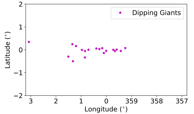
Figure 8. Locations of the 18 dipping giants in the Nuclear Disc. A 19th case is plotted at l = 3.1^\circ and two others lie a little further from the Galactic centre, at (l,b)=(350.7^\circ,-1.2^\circ) and (8.2^\circ,-0.2^\circ) , respectively.
