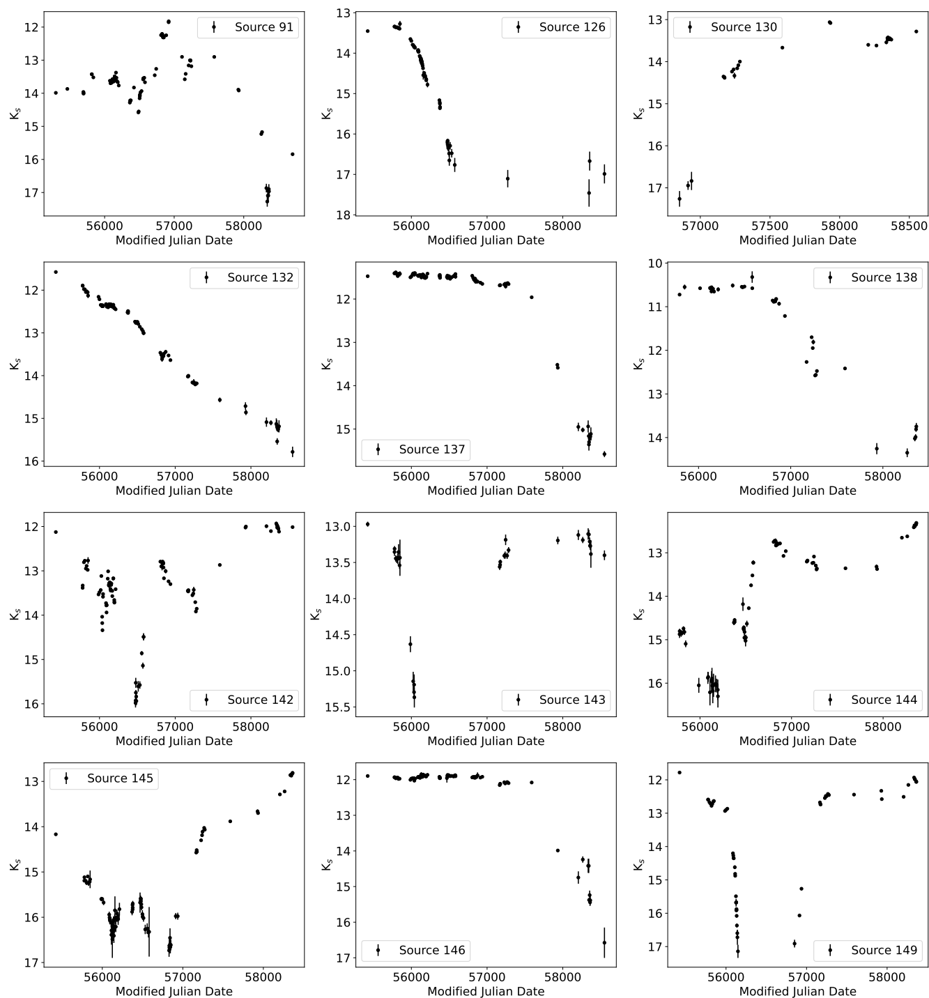
Figure 9. Light curves of the dipping giants
