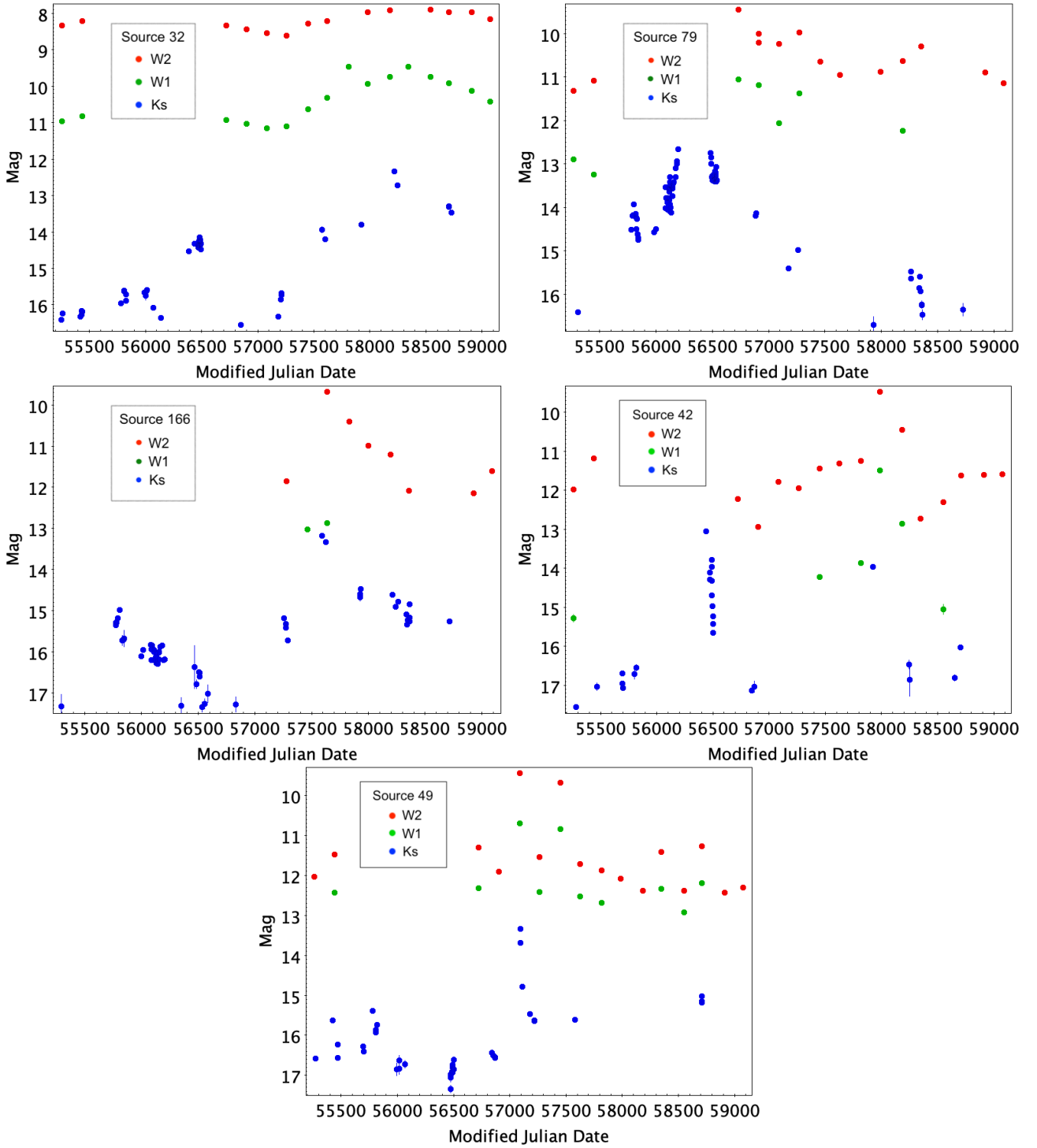
Figure D1. VVV and WISE light curves of five irregular eruptive YSOs.
